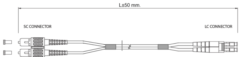
SC to LC FIBER OPTIC PATCH CORD DUPLEX
