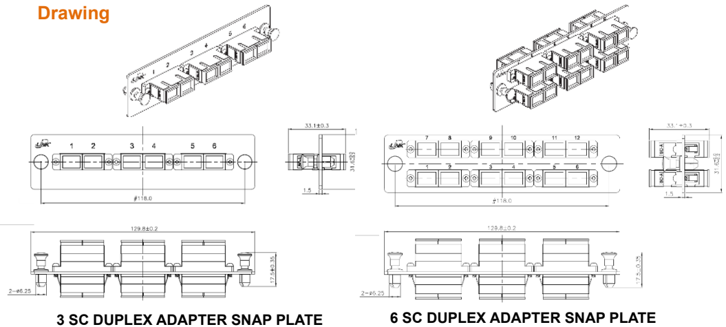
3 SC DUPLEX ADAPTER SNAP PLATE
